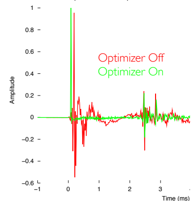
Impulse Response
