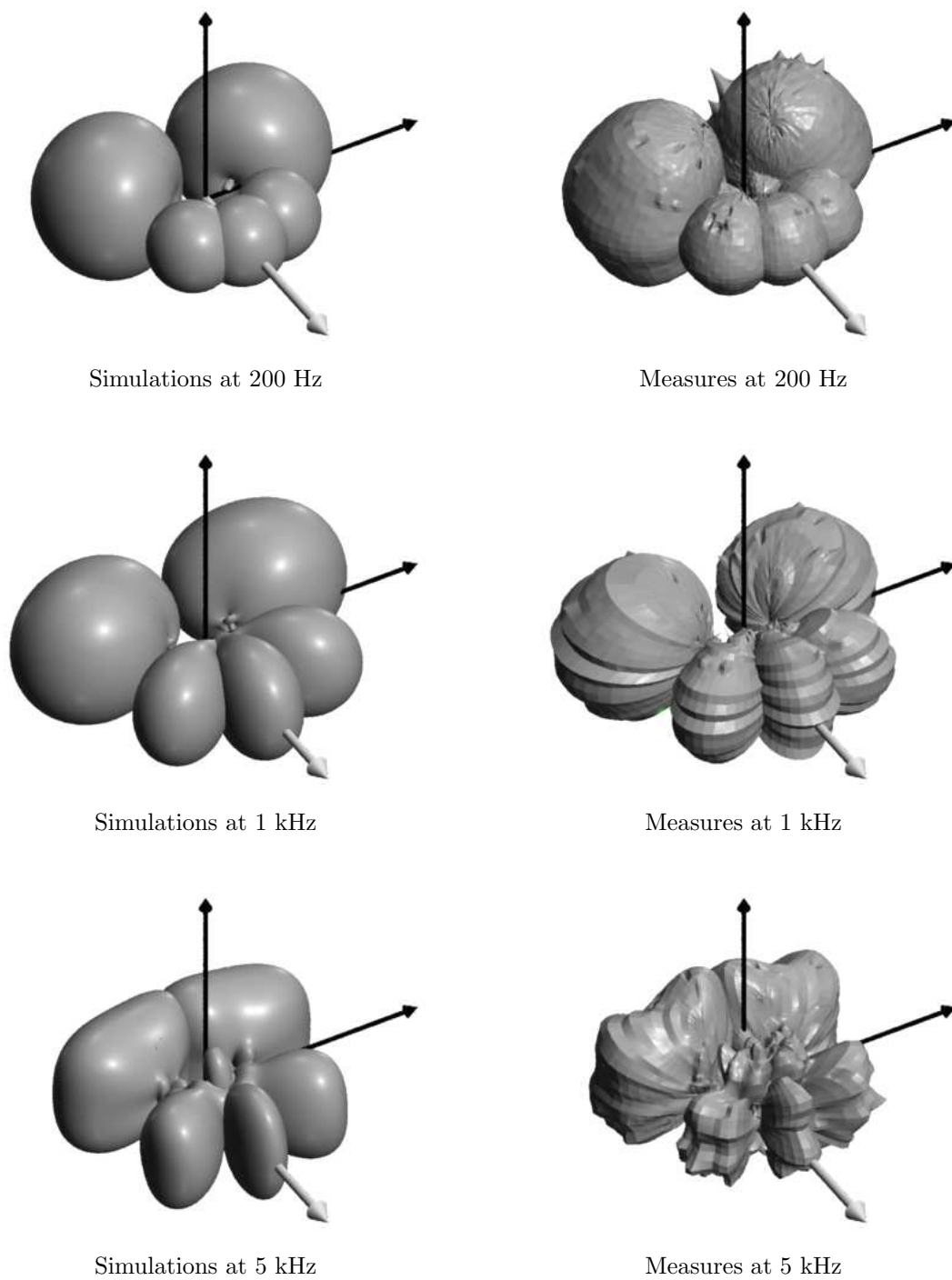
Fig. 19: Simulated and measured directivities obtained with the oblate omni filters.
