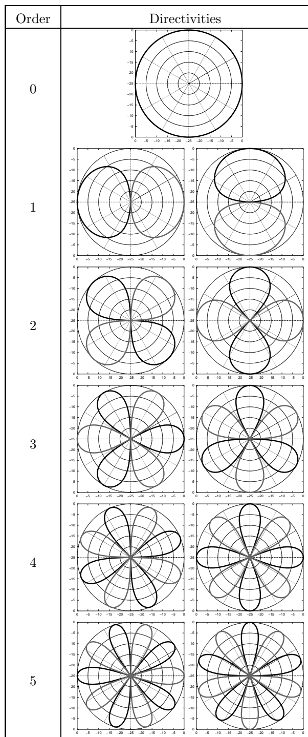
Fig. 6: Spatial frequencies until order 5. Negative lobes are in grey.
