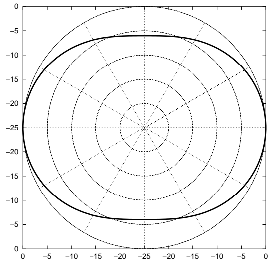
Global directivity in the vertical plane
