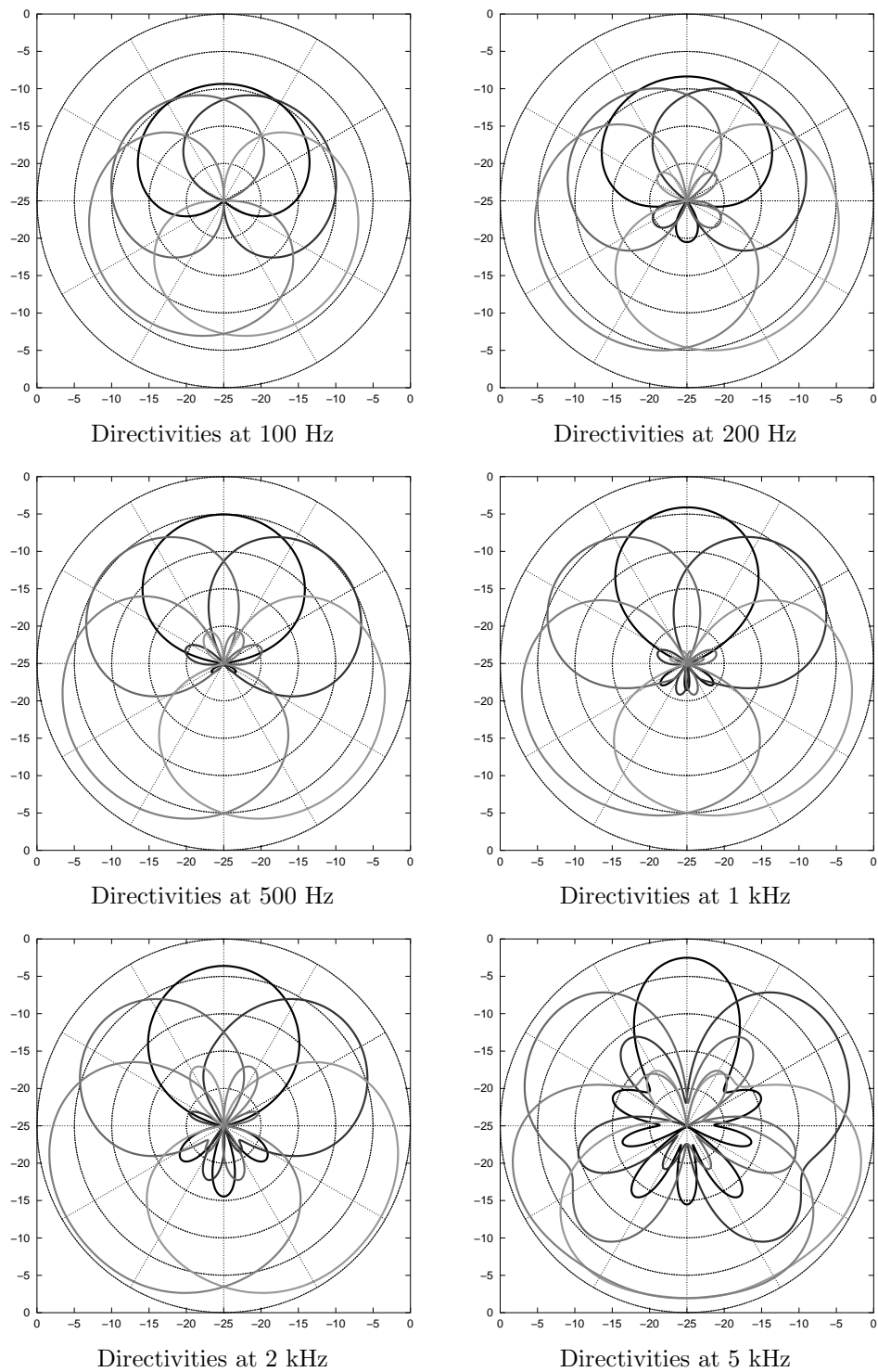
Fig. 18: Simulated directivities obtained with the omni filters.
