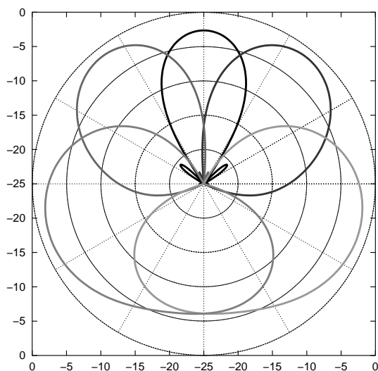
Fig. 4: 5th-order intensity panning law (cf. appendix A).
