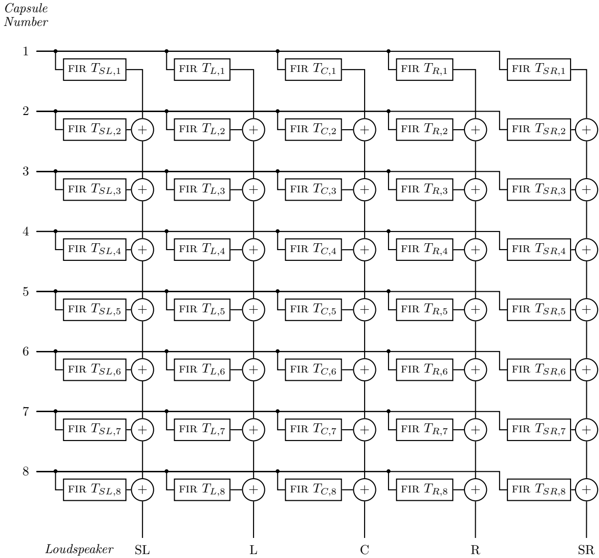
Fig. 9: Full Matrix Filtering.
