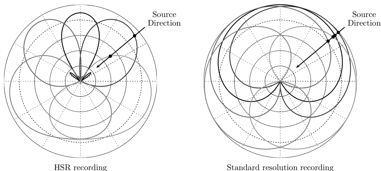
Fig. 16: Comparison between the recording of a source using HSR and using standard resolution.
