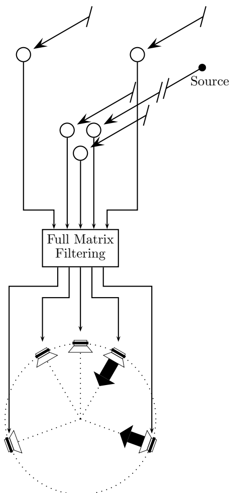
Fig. 10: Full-Matrix-Filtering-based 5.0 multichannel microphone.
