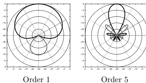
Fig. 7: Comparison of spatial resolutions of order 1 and 5.
