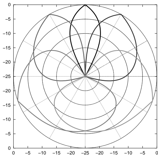
Fig. 3: Intensity panning law.
